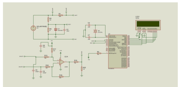
Fig 2. Circuit diagram for solar energy measurement system
