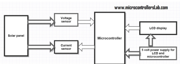
Fig. 1. Block diagram of solar energy measurement system
