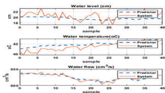
Figure 8. System respond
