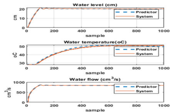
Figure 2. Normal system
