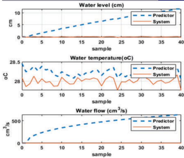
Figure 4. System respond
