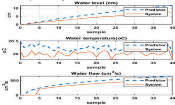
Figure 6. System respond
