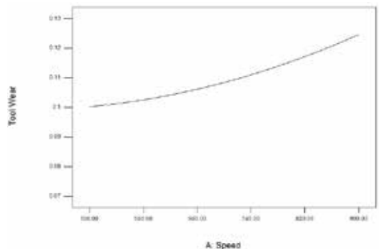
Figure 4. Effect of spindle speed on Tool wear
