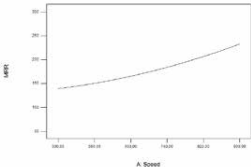
Figure 1. Effect of spindle speed on MRR
