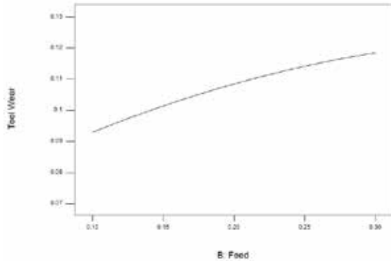
Figure 5. Effect of feed rate on Tool wear
