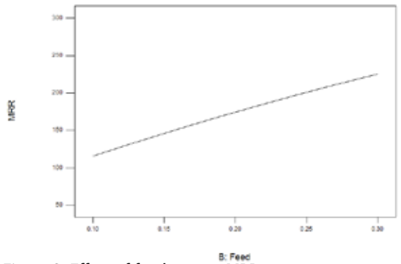
Figure 2. Effect of feed rate on MRR
