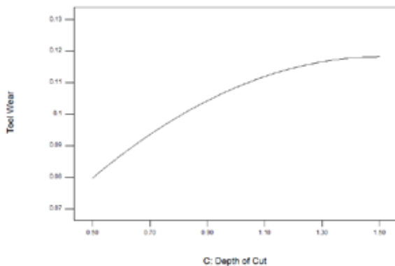
Figure 6. Effect of depth of cut on Tool wear
