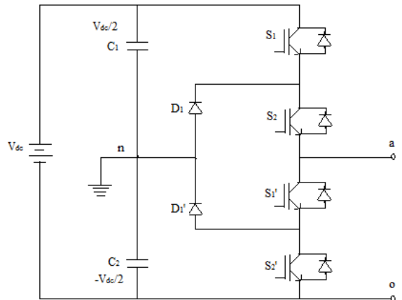
Fig: - 1 Three Level Diode Clamped inverter
