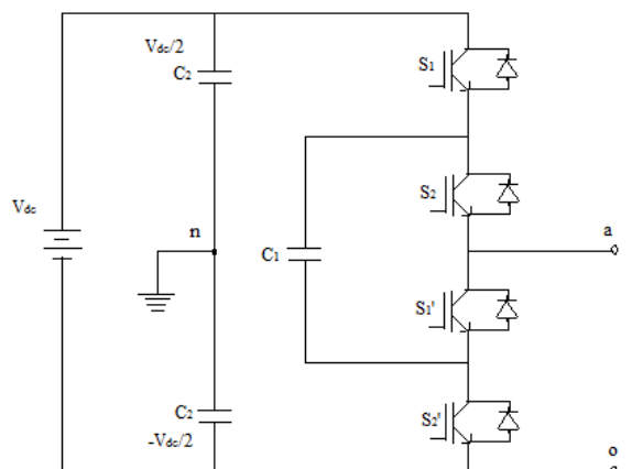
Fig: - 2 Three Level Capacitor Clamped inverter
