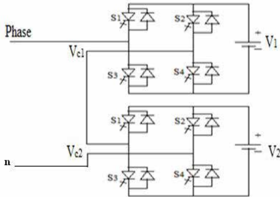
Fig: - 3 Three Level Cascaded inverter
