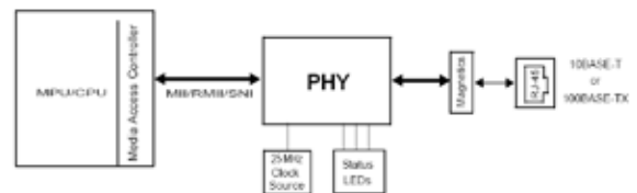
Fig.3.Microcontroller to Ethernet RJ45 jack Diagram
