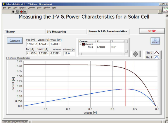
Figure 5. LabView interface program
