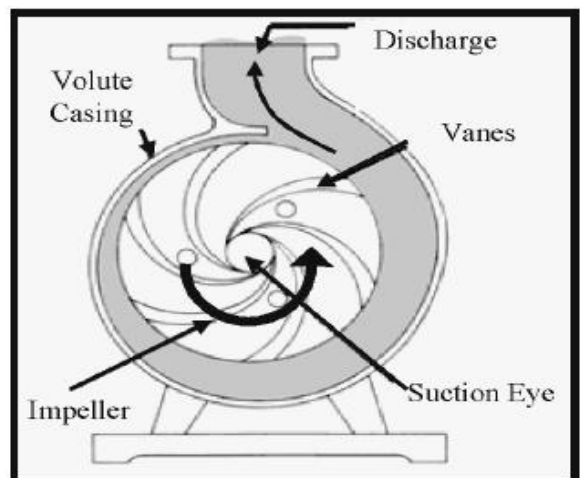
Figure 1 Centrifugal Pump
