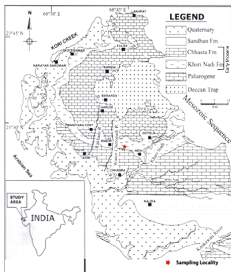
Fig. 1. Location and Geological map of the study area, Kachchh (after Biswas, 1992)
