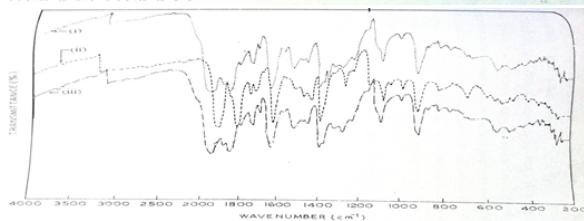
Fig. (3) (A) IR SPECTRA OF COMPLEXES
