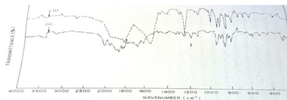
Fig. (3) (A) IR SPECTRA OF ORGANIC COMPOUNDS
