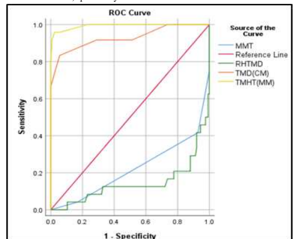
Figure 1 Receiver operating characteristic (ROC) curve for TMHT, TMD, RHTMD and MMT
