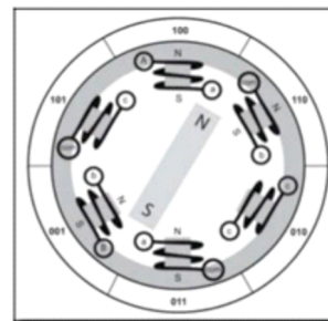
Fig.1. BLDC Motor Star Connected.
