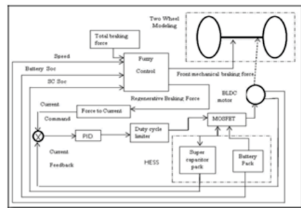
Fig.5 Proposed control strategy system
