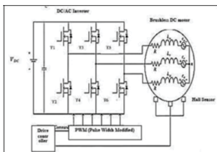
Fig.3 BLDC control by H-Bridge inverter
