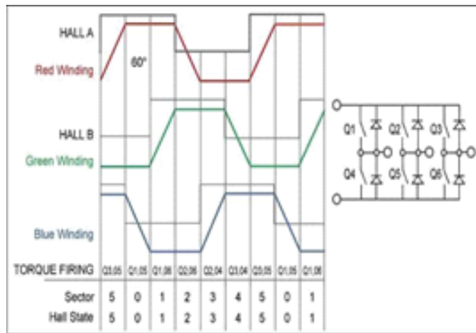
Fig.2 Back EMF BLDC motor phase
