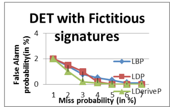
Fig. 5 – Plots LBP, LDP, and LDerivP
