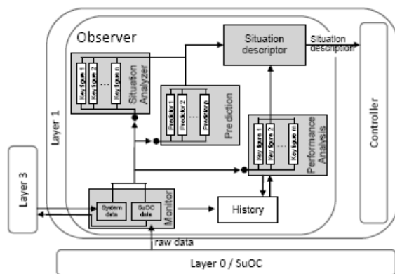
Figure 3: An observer/controller architecture for traffic signal control [20]
