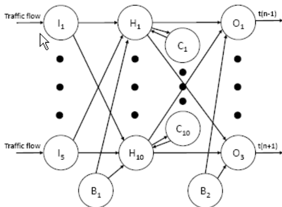
Figure 2: Structure of the neural network
