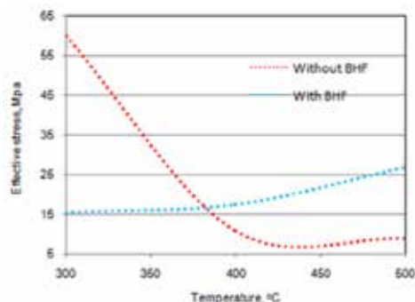
Fig-4. Influence of temperature on the effective stress.
