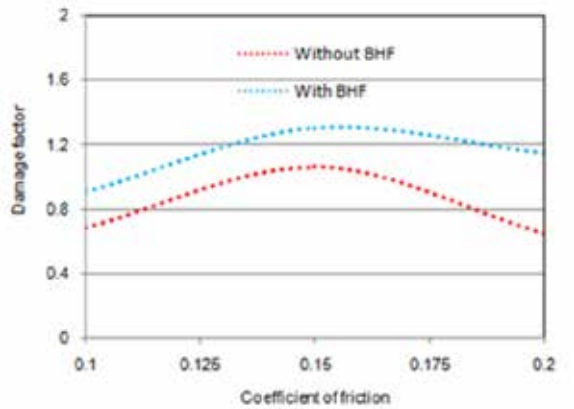
Fig-19. Influence friction on the damage of cup.
