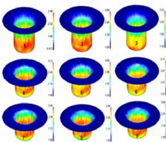
Fig-17. Surface expansion ratio of cups without BHF.
