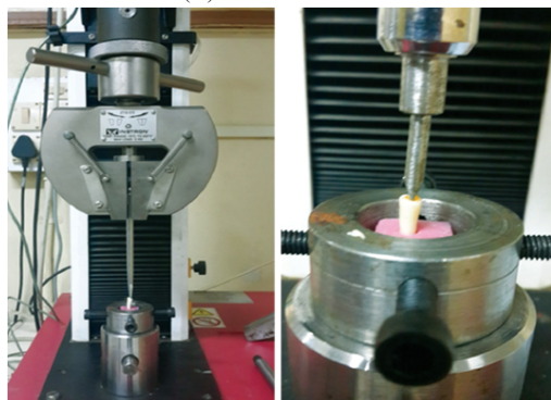
Fig. 1: Samples mounted on Universal Testing Machine
