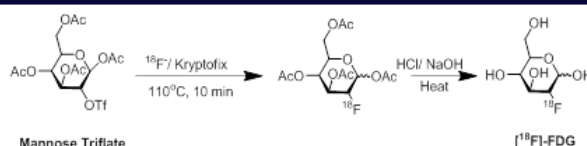
Scheme 2. Radiosynthesis of [ ^{18}\text{F} ]-FDG by nucleophilic substitution.
