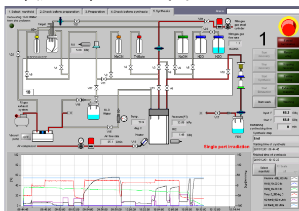
Figure 5:- Schematic diagram of the automated synthesis of ^{18}\text{F} -FDG of F300E synthesizer
