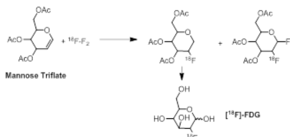
Scheme 1. Radiosynthesis of [ ^{18}\text{F} ]-FDG by electrophilic substitution.
