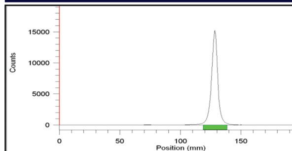
Figure 9: Radio TLC scan chromatogram
