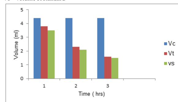
Fig. 9. Anti-Inflammatory studies.
