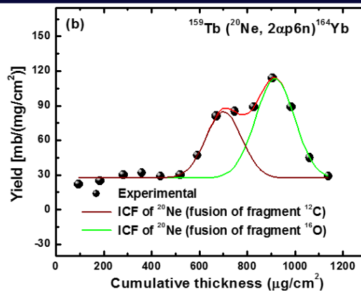
Fig.2: The experimentally measured FRRD of ER ^{164}\text{Yb} produced via ICF for ^{20}\text{Ne} + ^{159}\text{Tb} system at energy, E \sim 164 MeV.
