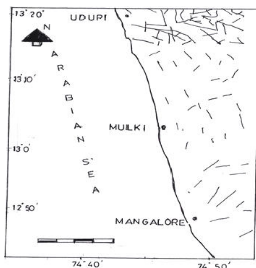
Figure 5. Lineaments of Southern Coastal Karnataka
