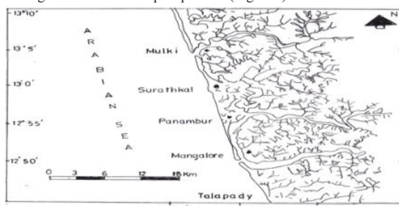
Figure 2. Drainage Pattern: Southern Coastal Karnataka
