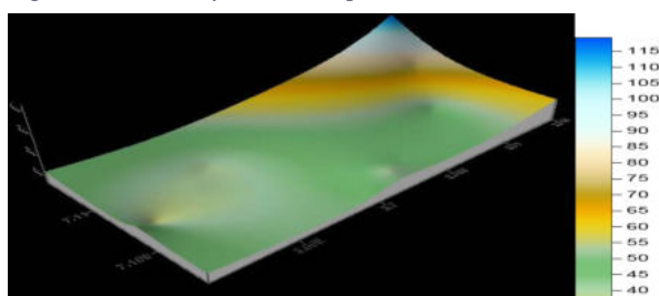
Figure 4: Isoresistivity Contour Map of VES Stations on Granite Gneiss.
