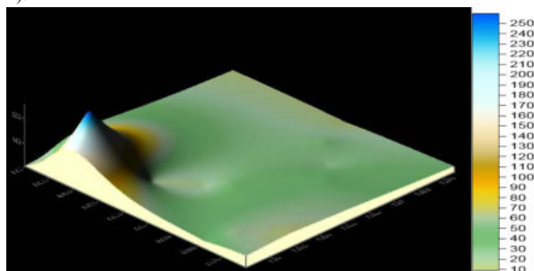
Figure 2: Isoresistivity Contour Map of VES Stations on Granite Gneiss.
