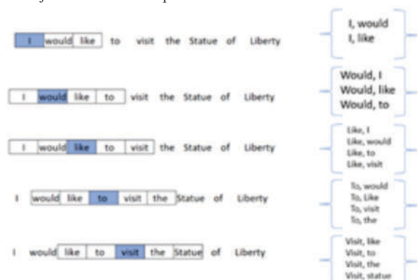
Figure -2: A skip gram model explanation
