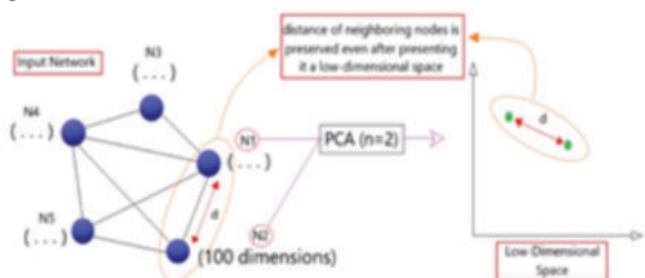
Figure-4: Dimension reduction in node2vec
