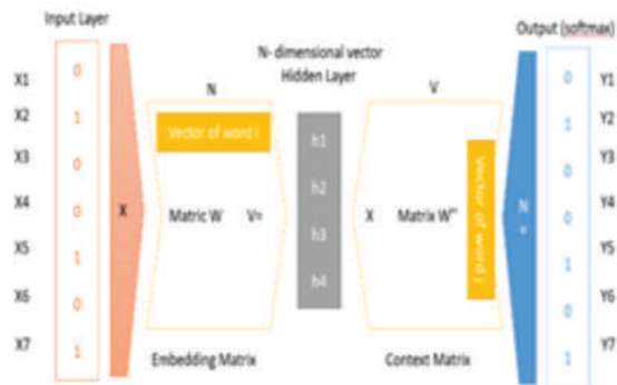
Figure-3: A skip gram model architectural diagram
