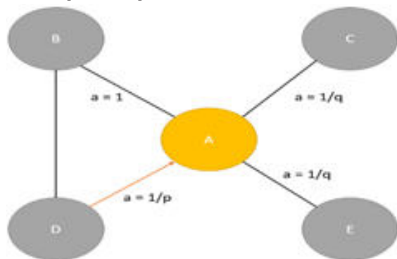
Figure-8: Second order random walk
