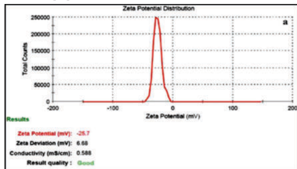
Figure 1: Zeta potential of niosomal formulation (F4).
