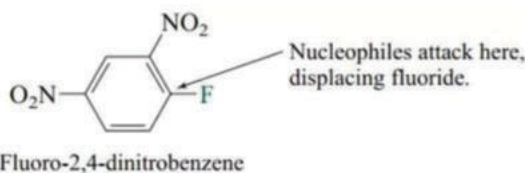
Figure 10: structure of 1-fluoro-2, 4-dinitrobenzene
