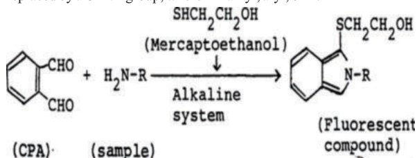
Figure 12: Scheme for hydrolysis reaction with amines
