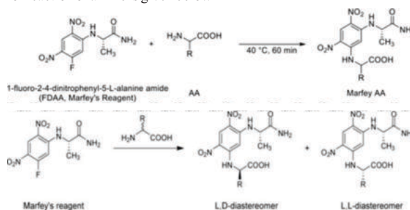
Figure 11: Scheme for substitution reaction of FDAA and formation of diastereomers Pregabalin also contain primary amine which makes it fit for this reaction. Hence the molecule was explored for this purpose. The pregabalin is allowed to react with marley's which gives derivative of pregabalin. [36-39] In this study solution of pregabalin was prepared by weighing 80 mg of Pregabalin and dissolved in 2 mL of 1mol/L HCl (pH was set to 7.0 with NaOH solution, up to 10 mL by distilled water.
