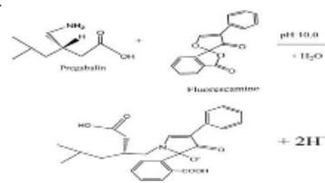
Figure 14: Scheme for reaction of fluorescamine with Pregabalin
