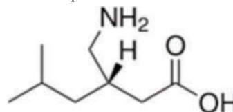
Figure 1: Structure of Pregabalin
