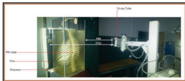
Fig. 2. The experimental set-up
