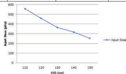
Fig. 4. Graph showing the reduction in input dose due to an increase in Film-Focus Distance (FFD)
