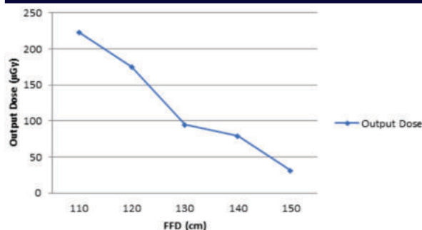
Fig. 5. Graph showing the reduction in Output dose due to increase in Film-Focus Distance (FFD)
