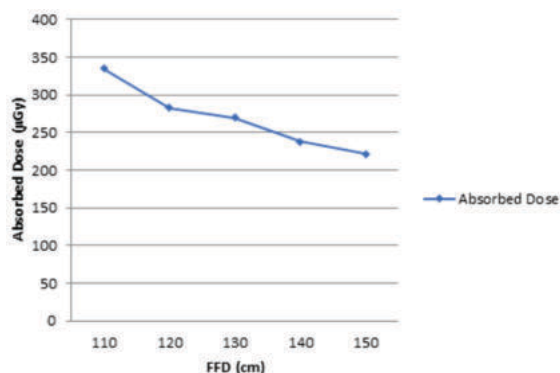
Fig. 6. Graph showing the reduction in Absorbed dose due to an increase in Film-Focus Distance (FFD)
