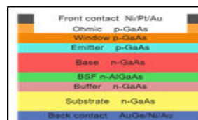
Fig. 2(b) GaAs solar cell
