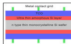
Fig. 2(a) Heterojunction Intrinsic Thin layer solar cell
