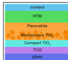
Fig. 3(a) Perovskite solar cell
