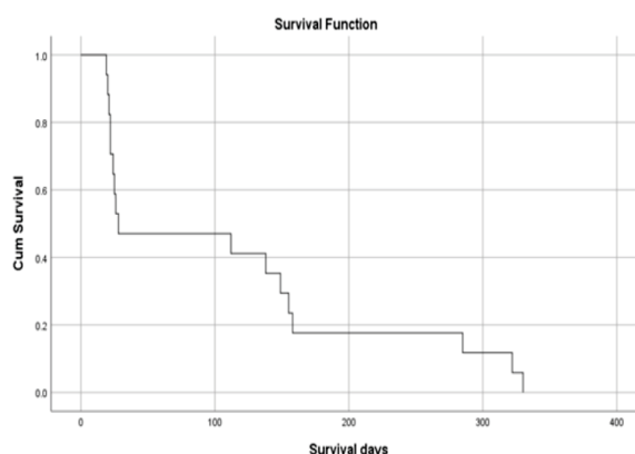
Figure 1: Cumulative Survival Curve
