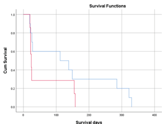
Figure 2: Age Group Related Survival Curve
