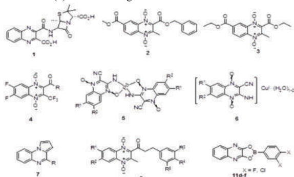
Fig. I: Biologically Potent Quinoxaline Derivatives.
