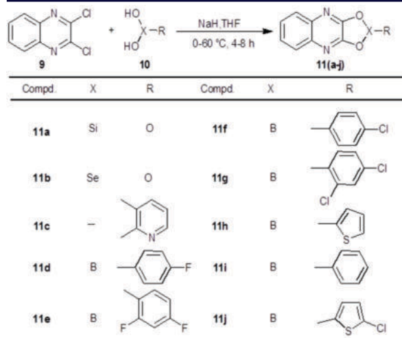
Scheme 1: Synthesis of boron, silicon and selenium substituted quinoxaline derivatives 11(a-j).
