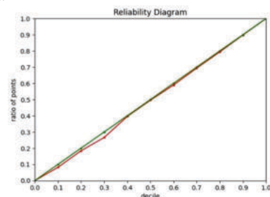
Figure 1: Reliability Diagram For Heteroskedastic Regression
