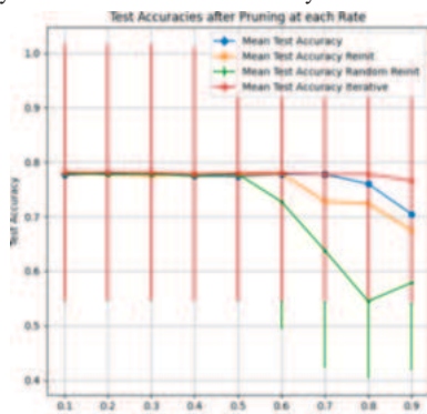
Figure 5: Accuracy vs. Pruning Ratio for MakeMoons Dataset
