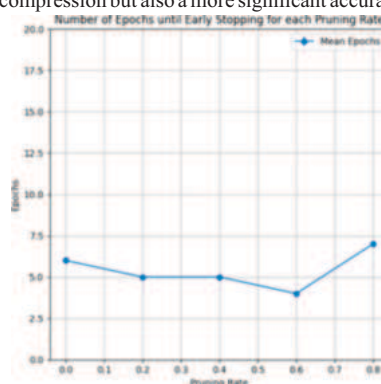
Figure 6: Early-Stop Iteration (Val.) vs. Pruning Ratio for Cifar10 Dataset
