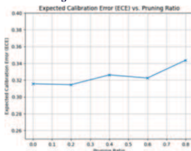
Figure 9: ECE vs Pruning Ratios for CIFAR 10 Dataset
