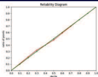
Figure 2: Reliability Diagram For Homoskedastic Regression
