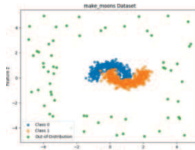
Figure 3: MakeMoons Dataset
