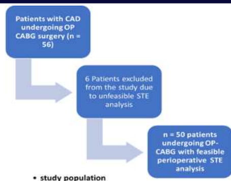
Figure 1 Study Population
