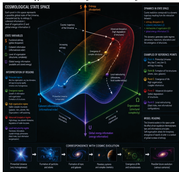
Figure 2: Summary of the Cosmological Model
