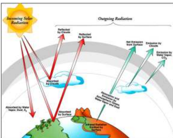
Figure – 1.1 Natural solar radiation on earth {source : [1]}
