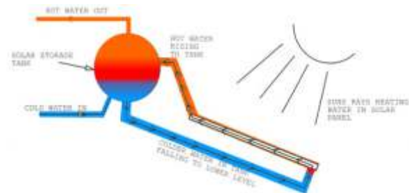
Figure – 5.1 Natural thermosyphonic type flat plate collector water heater flow process (source : www.mnre.gov.in )
