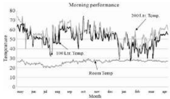
Figure 6.1 - Solar water heater performance (morning).
