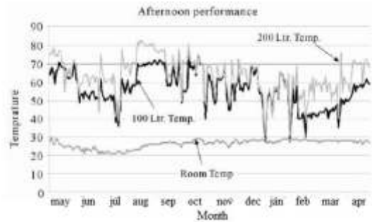
Figure 6.2 - Solar water heater performance (afternoon).
