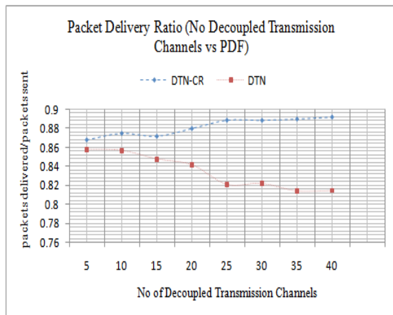
Fig1: Evaluating the Throughput explored by DTN with CR and DTN by Binary Spray and wait strategy
