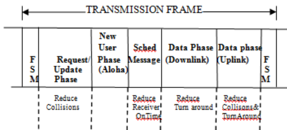
Figure 1. EC-MAC protocol frame protocol frame structure.
