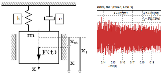
Fig.1. System model of 1 degree of freedom and vibration signal of real system
