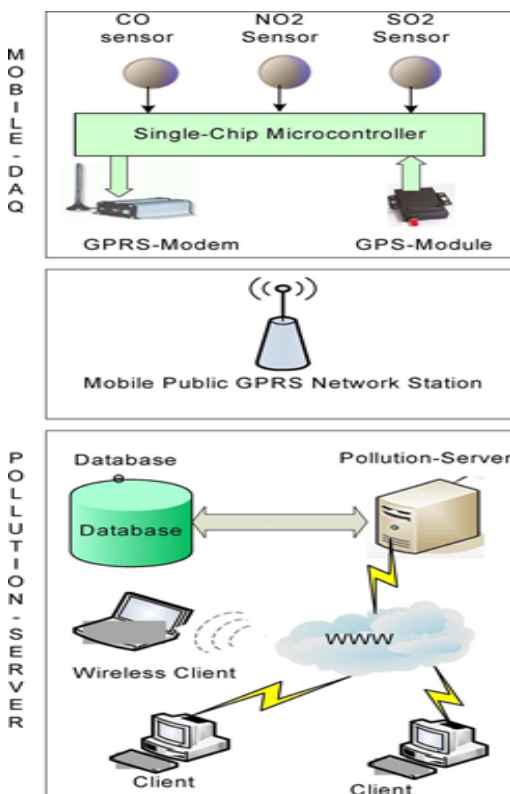
Fig. 1. System hardware basic building blocks.
