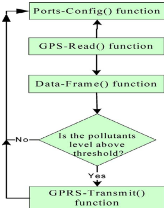
Fig. 3. Mobile-DAQ software algorithm.
