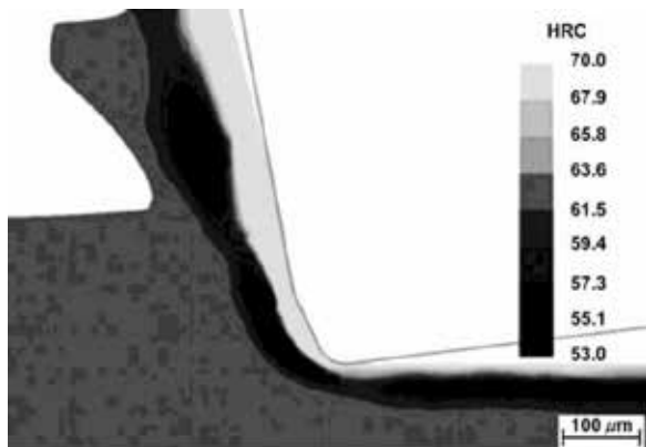
(b) Fig.2. Observed (a) and simulated (b) white and Dark layers formation and initial hardness 53 HRC, Reprinted with permission from [9].
