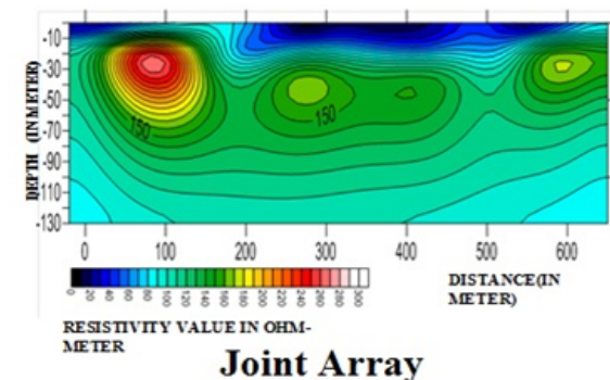
Fig. 5. Plot of Joint Array
