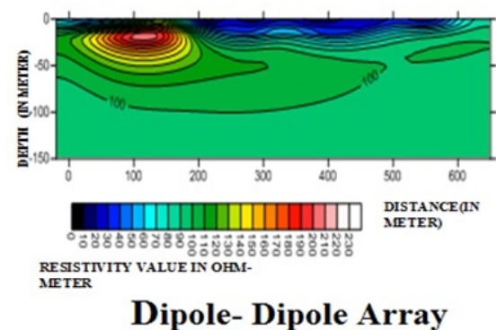
Fig.4. Plot of Dipole-Dipole Array
