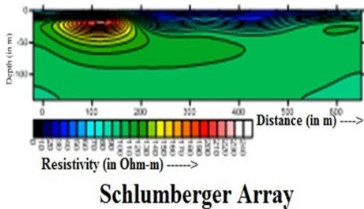
Fig.3. Plot of Schlumberger array
