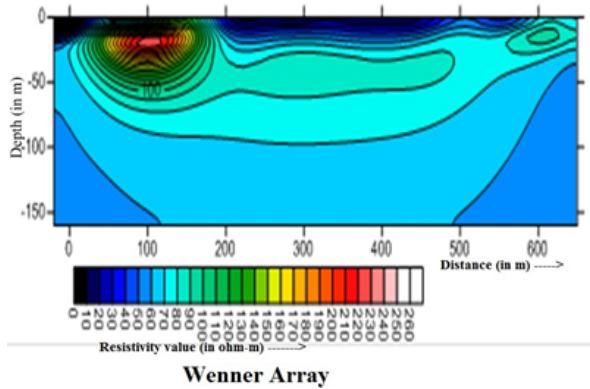
Fig.2. Plot of Wenner Array
