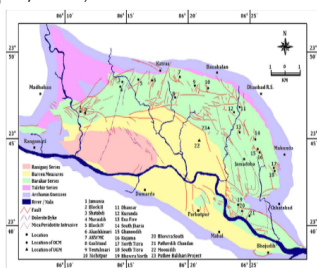
Fig.1. Geological map of Patherdih area with stratigraphic succession
