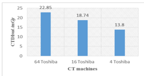
Figure 4: Shows the comparison between the CTDIvol for the CT KUB procedure in the three hospitals by three Machines.
