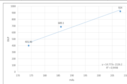
Figure 1: shows the relation between the DLP and mAs for CT KUB procedure in the three hospitals by three machines.
