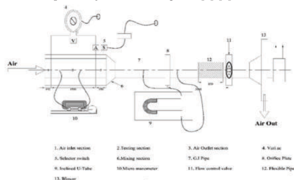
Figure 1 A schematic view of setup of SAH
