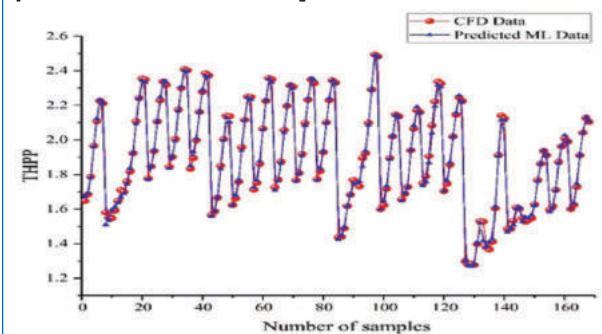
Figure 2. Comparison of computational fluid dynamics (CFD) results with predicted values of THPP
