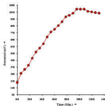
FIG. 1 VARIATION OF POTENTIAL WITH TIME
