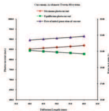
Fig. 3 VARIATION OF CURRENT PARAMETERS WITH DIFFUSION LENGTH
