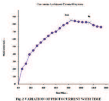
Fig. 2 VARIATION OF PHOTOCURRENT WITH TIME
