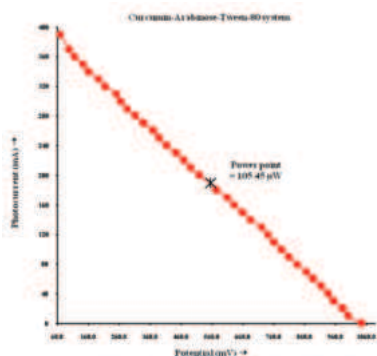
Fig. 4 CURRENT VOLTAGE (I-V) CURVE OF THE CELL
