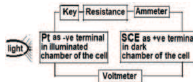
Fig. 7 Photogalvanic Cell Set-up
